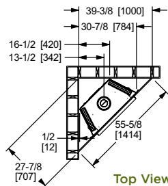
Top View Corner Installation
